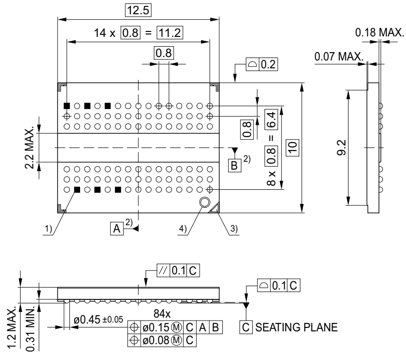
FIGURE 12 Package Outline P(G)-TFBGA-84
