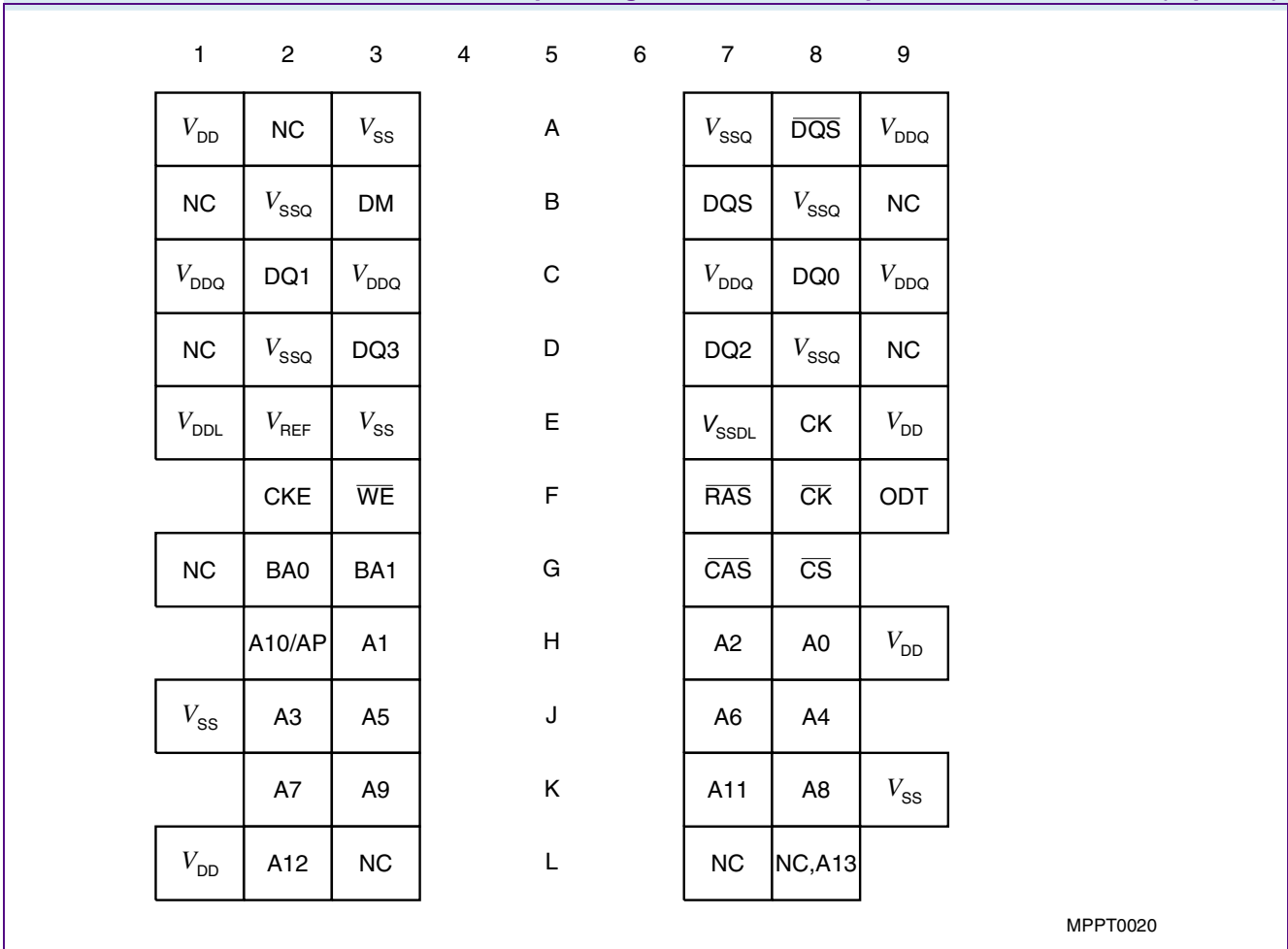
FIGURE 1 Chip Configuration for ×4 components, PG-TFBGA-60 (top view)
